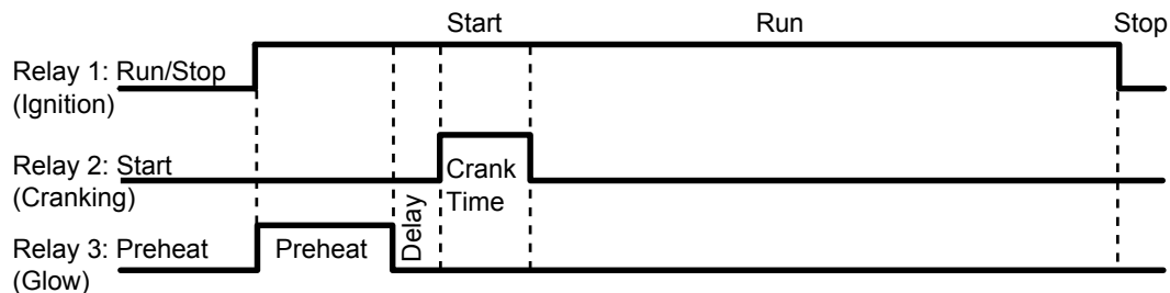
Figure 37 RunMode Timing Diagram
