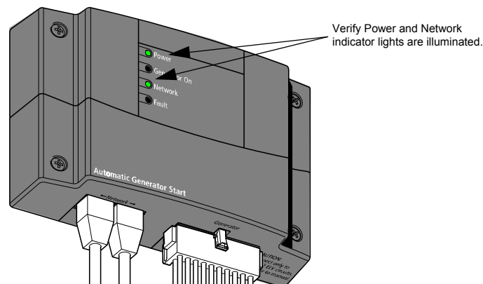
Figure 27 Verifying Power is Available
