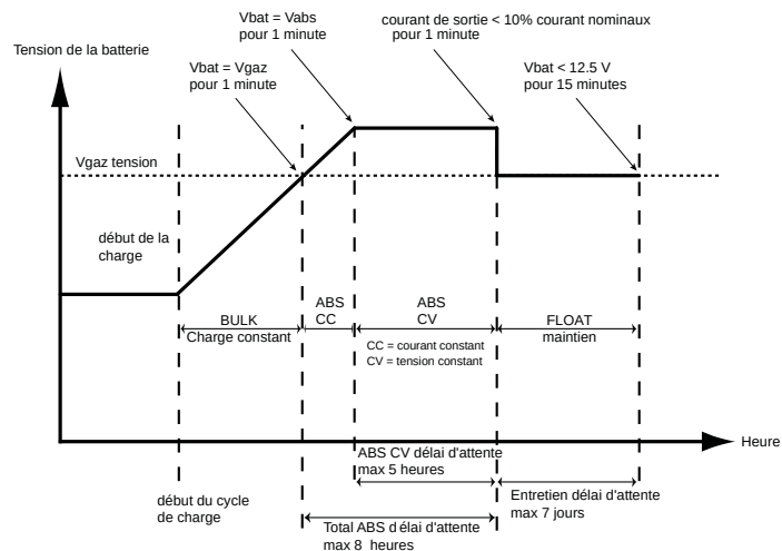
Figure 11 Cycle de charge en 3 Stage (trois phases)
