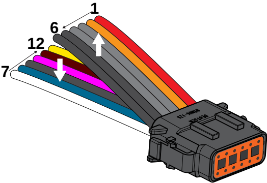
Figure 11 Deutsch connector harness
