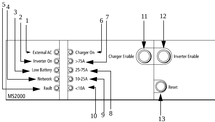
Figure 1-3 Front Panel Lights and Buttons
